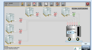
Resin Dispensing
